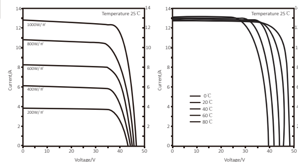
Current-Voltage Curve
